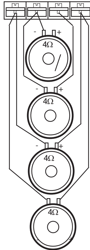
Connection of four subwoofers with 4 ohm single voice coil Impedance = 1 ohm
