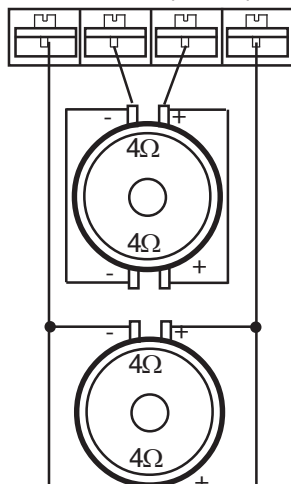
Connection of two subwoofers with 4 ohm dual voice coils Impedance = 1 ohm
