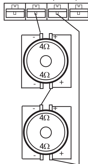
Connection of two subwoofers with 4 ohm dual voice coils in parallel and then in series to the amplifier with a resulting impedance of 4 ohms.
