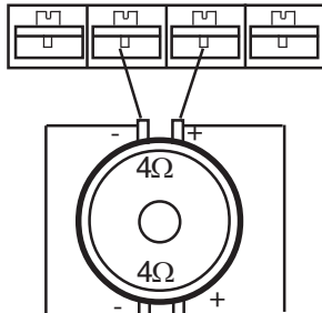
Connection of a subwoofer with 4 ohm dual voice coils Impedance = 2 ohm
